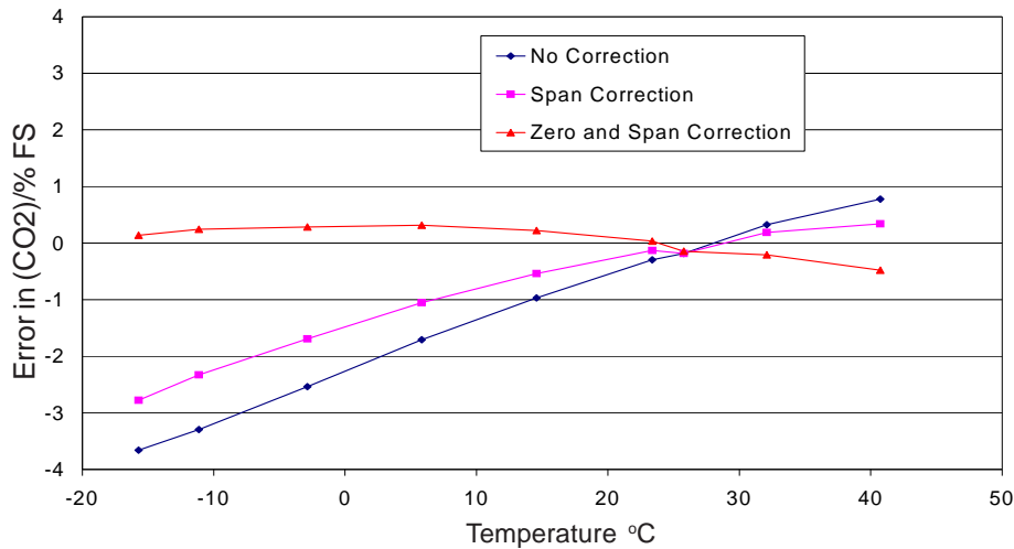
Figure 4 Temperature Compensation
