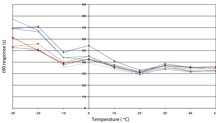
Figure 3 Response Time Temperature Dependence
