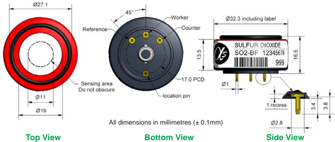
Figure 1 SO2-BF Schematic Diagram
