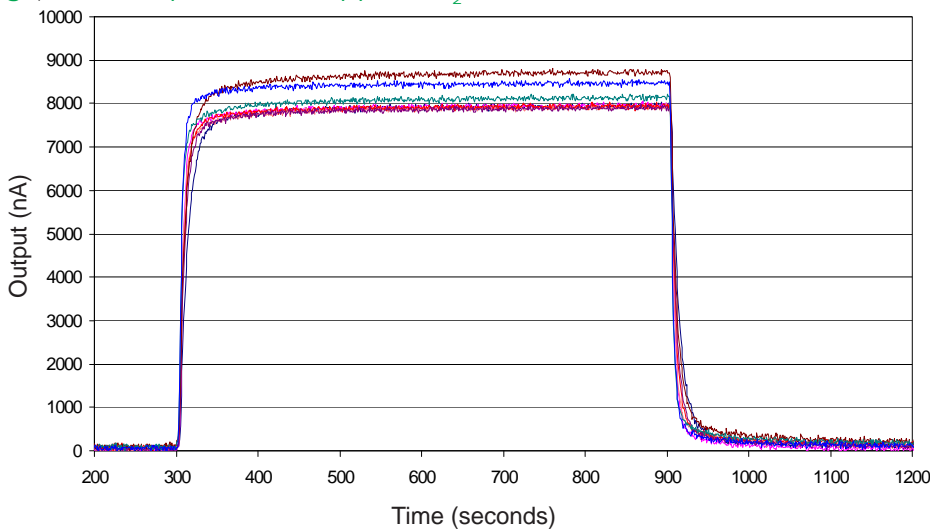
Figure 4 Response to 20ppm SO 2
