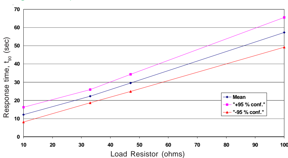
Figure 4 Response Time vs. Load Resistor
