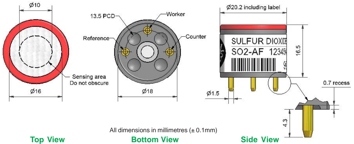
Figure 1 SO2-AF Schematic Diagram
