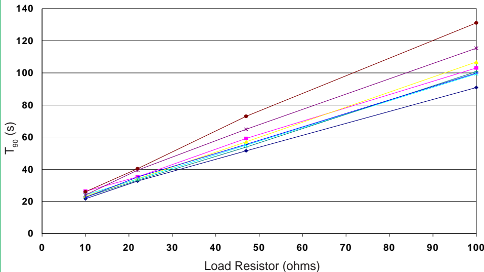
Figure 4 Effect of Load Resistor
