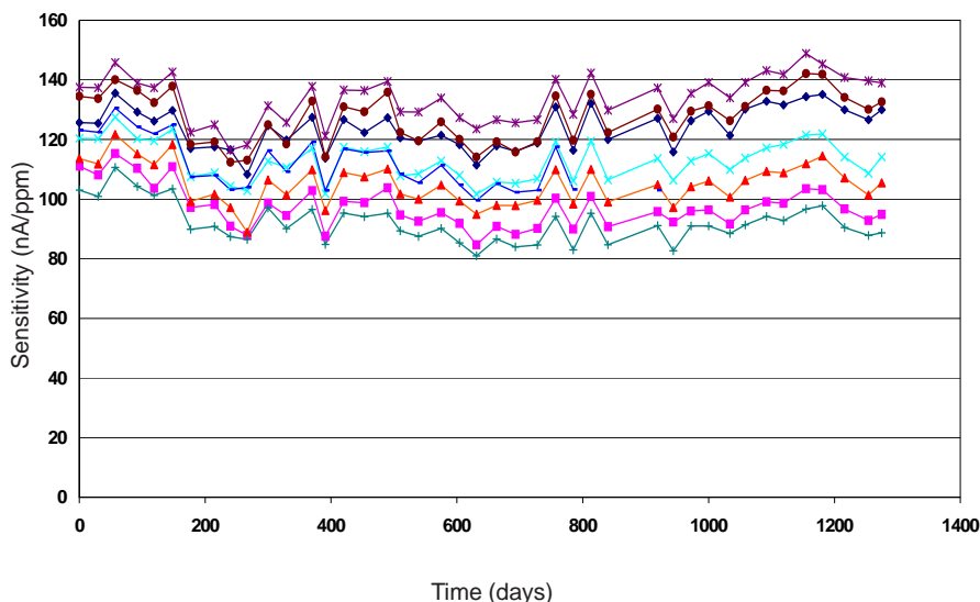
Figure 7 Ambient Long Term Test Results
