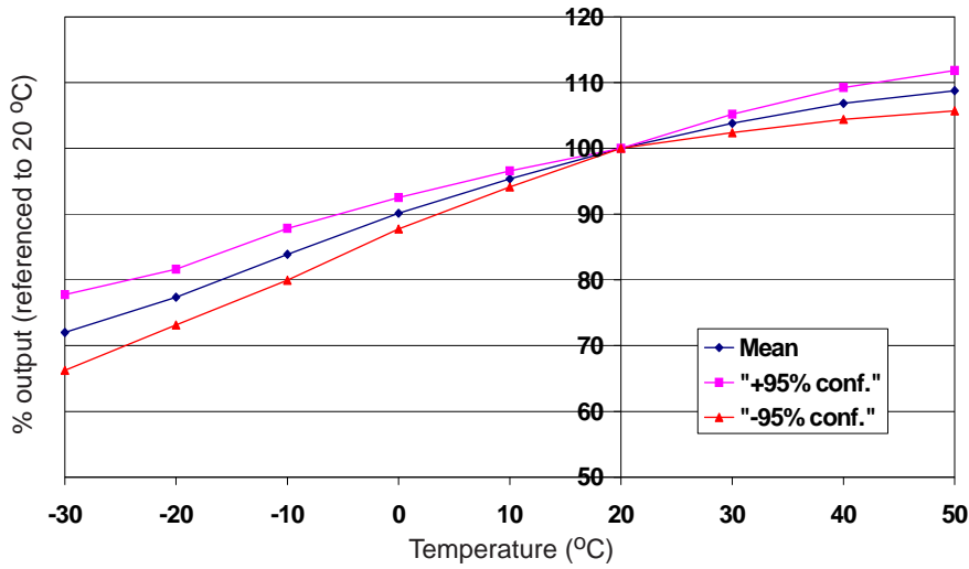
Figure 3 Hydrogen Temperature Dependence
