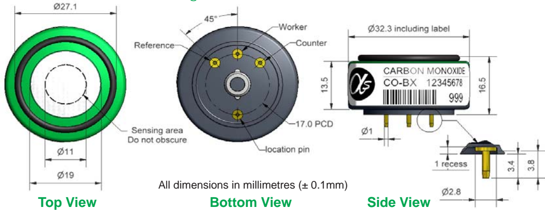
Figure 1 CO-BX Schematic Diagram
