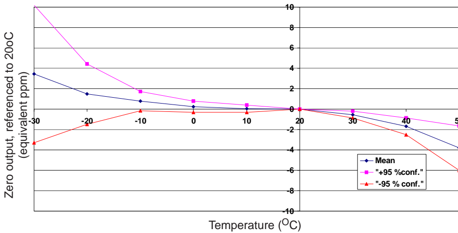
Figure 4 Hydrogen Temperature Dependence
